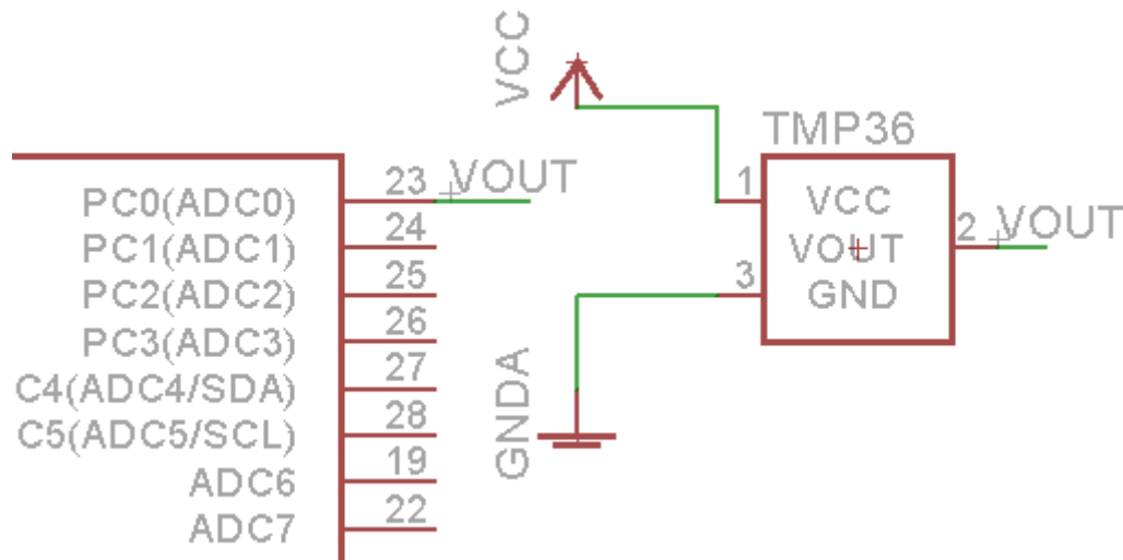
Figure 45: Temperature Sensor Connection Schematic
