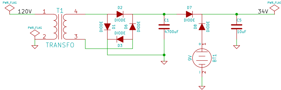
Figure 30: Power board AC rectification
