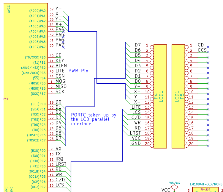
Figure 38: Base Station LCD header to MCU
