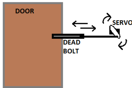
Figure 43: servo motor access control design
