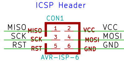
Figure 41: Base Station ISP header
