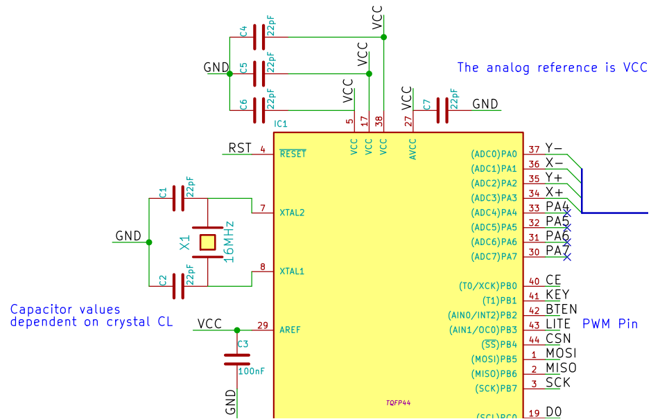
Figure 37: Base Station crystal and decoupling capacitors
