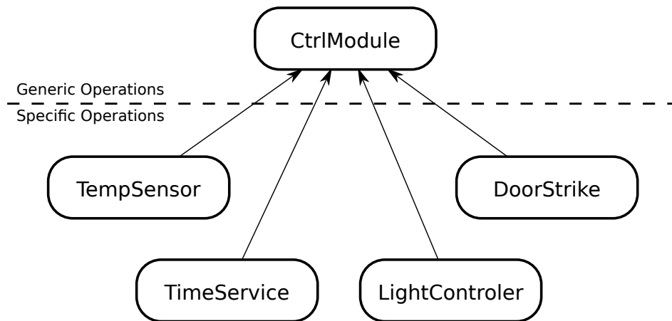
Figure 33: showing the control module hierarchy for WHCS
