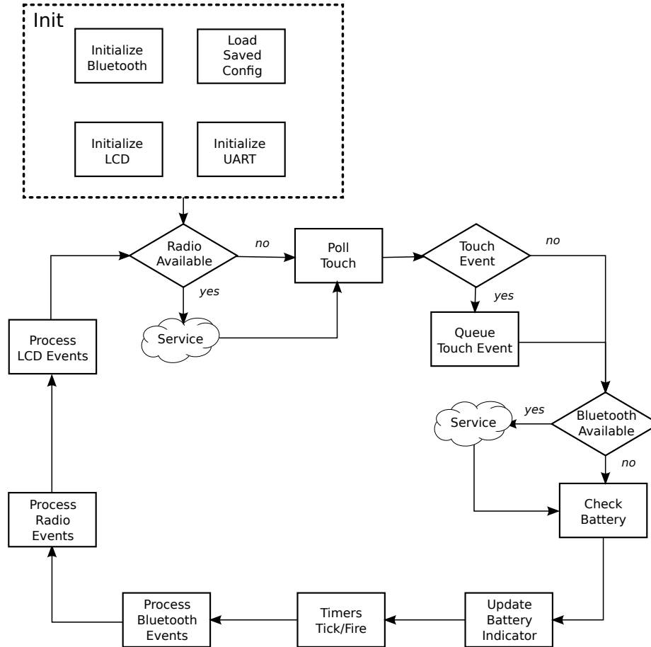
Figure 32: the high level software flow for the base station
