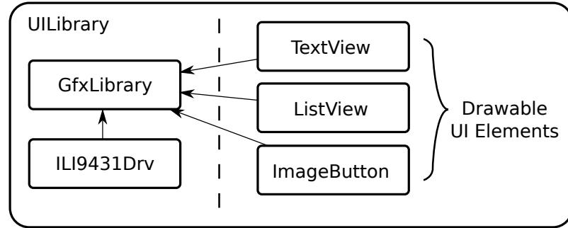
Figure 35: the level of abstractions for the LCD subsystem
