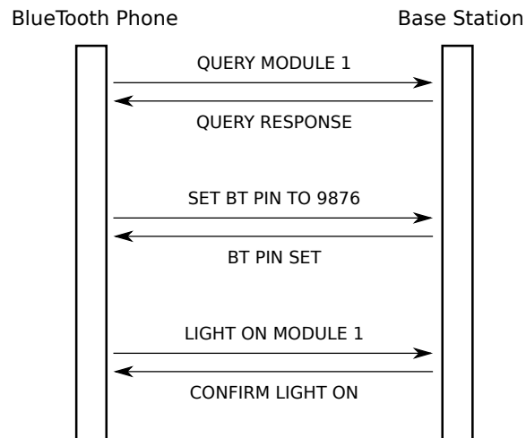
Figure 34: an example sequence diagram that could occur between a connected bluetooth phone and the base station
