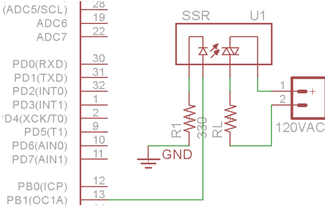
Figure 46: Wiring Schematic for Solid State Relay
