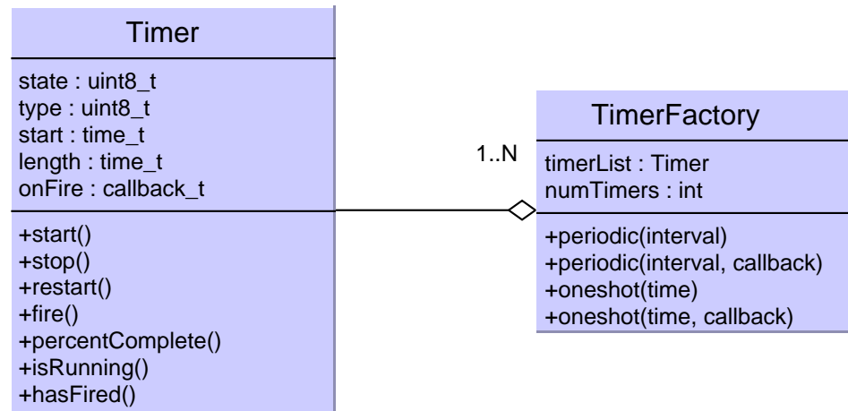
Figure 36: A UML representation of the Timer class
