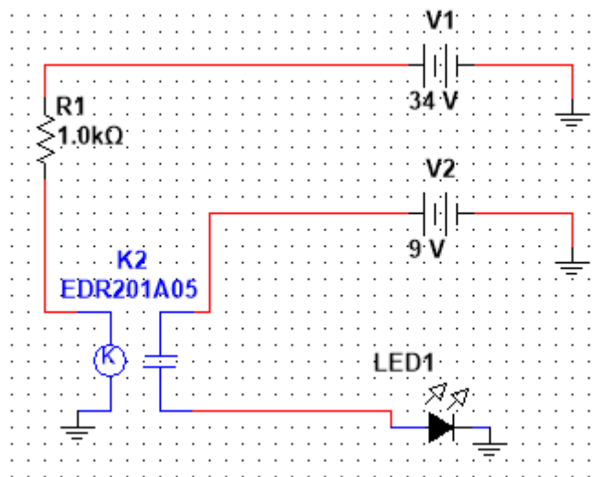
Figure 28: Possible design for back up battery[16]
