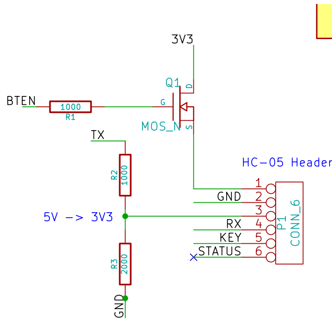
Figure 40: Base Station HC-05 header
