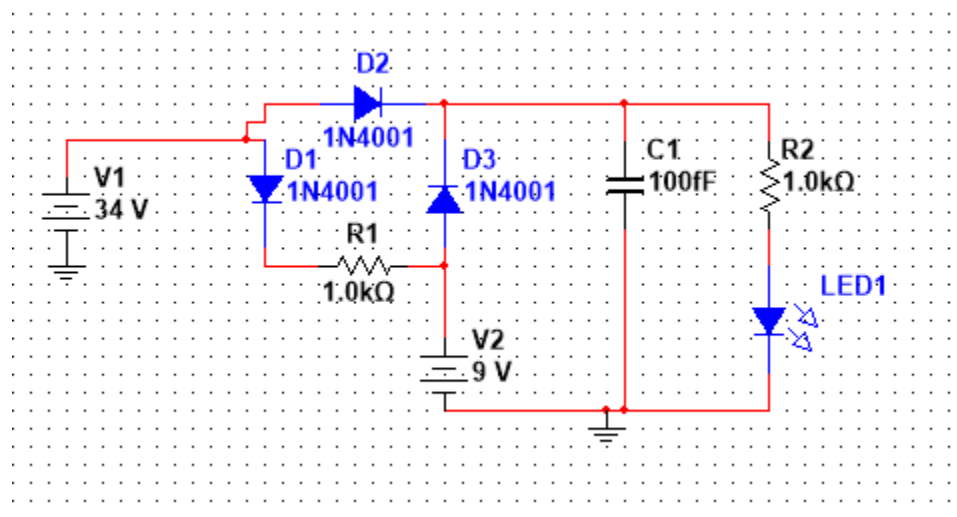
Figure 27: First possible design for the backup battery
