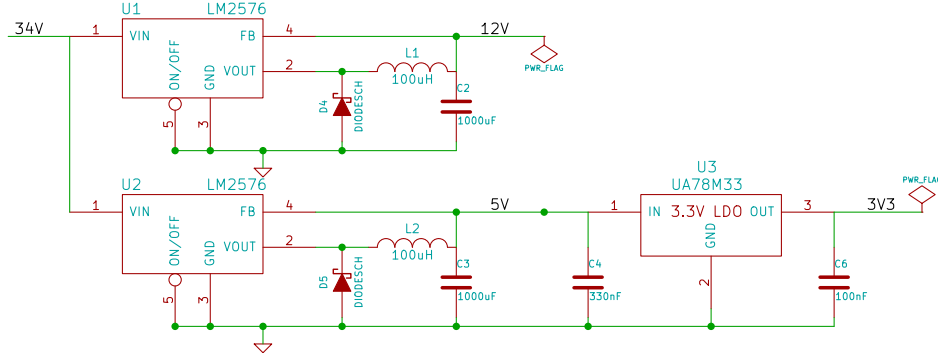
Figure 31: Power board AC rectification
