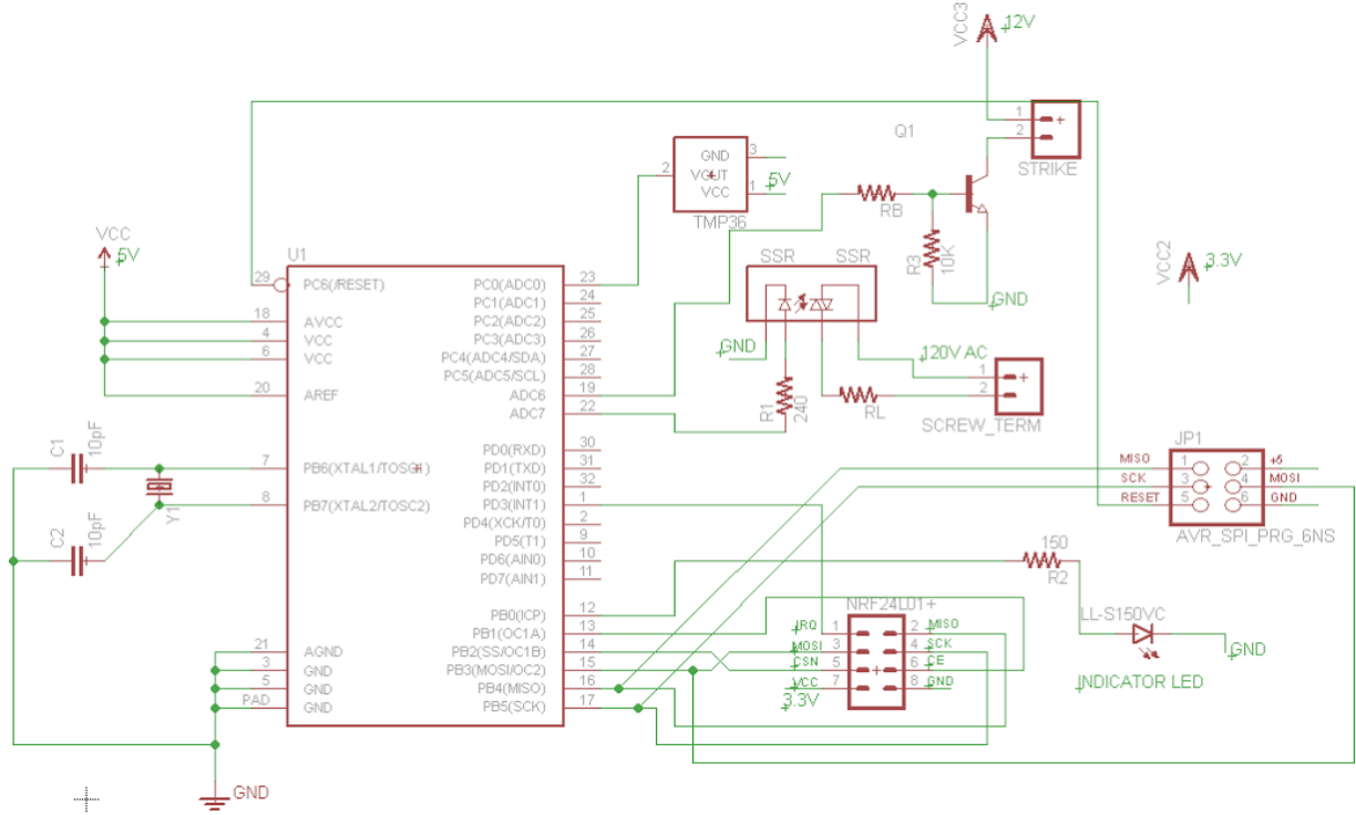
Figure 47: WHCS Control Module Schematic
